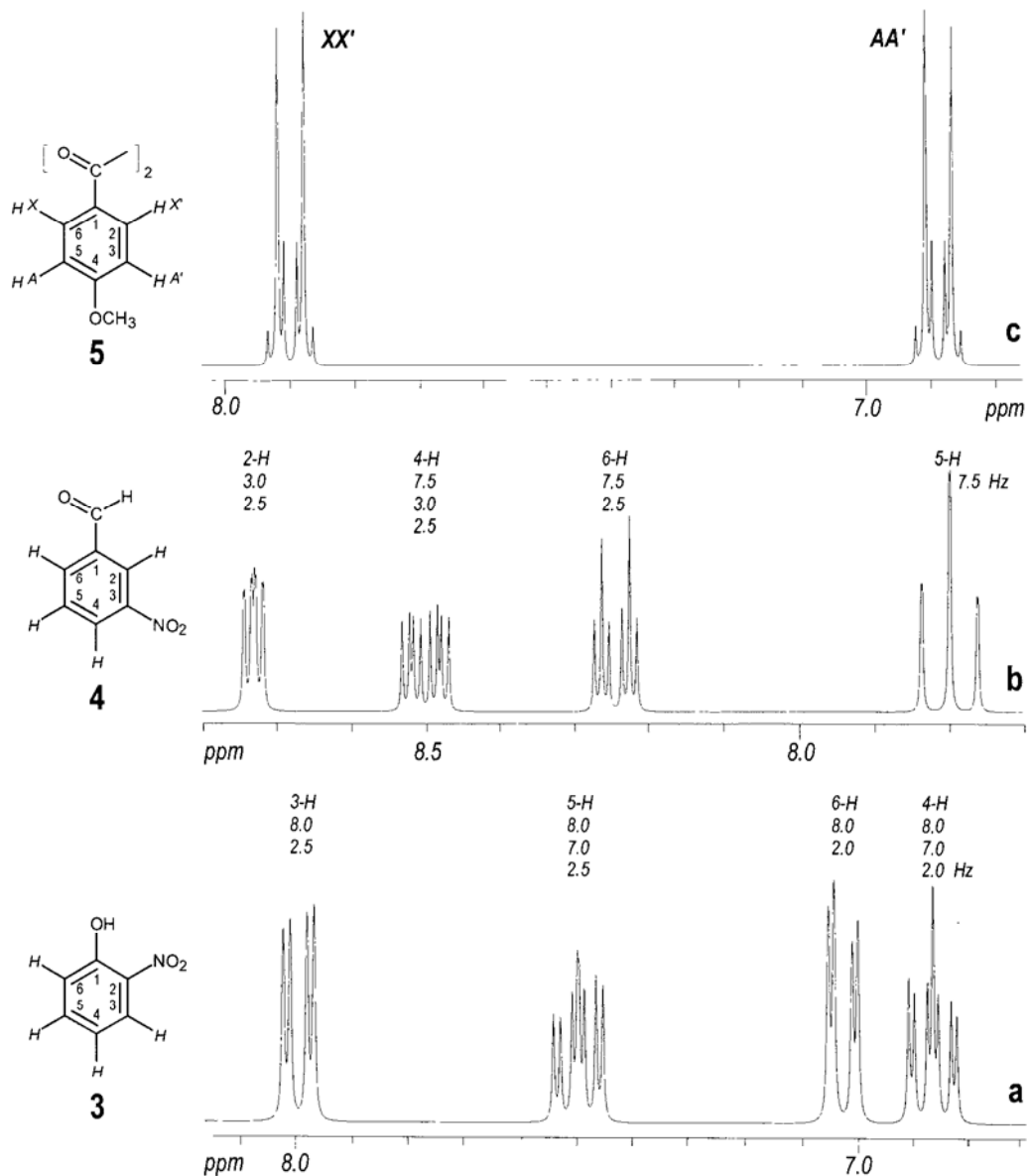
Figure 2.6. ^1H NMR spectra of disubstituted benzene rings [ CDCl_3 , 25 °C, 200 MHz]. (a) o -Nitrophenol ( 3 ); (b) m -nitrobenzaldehyde ( 4 ); (c) 4,4'-dimethoxybenzil ( 5 )
