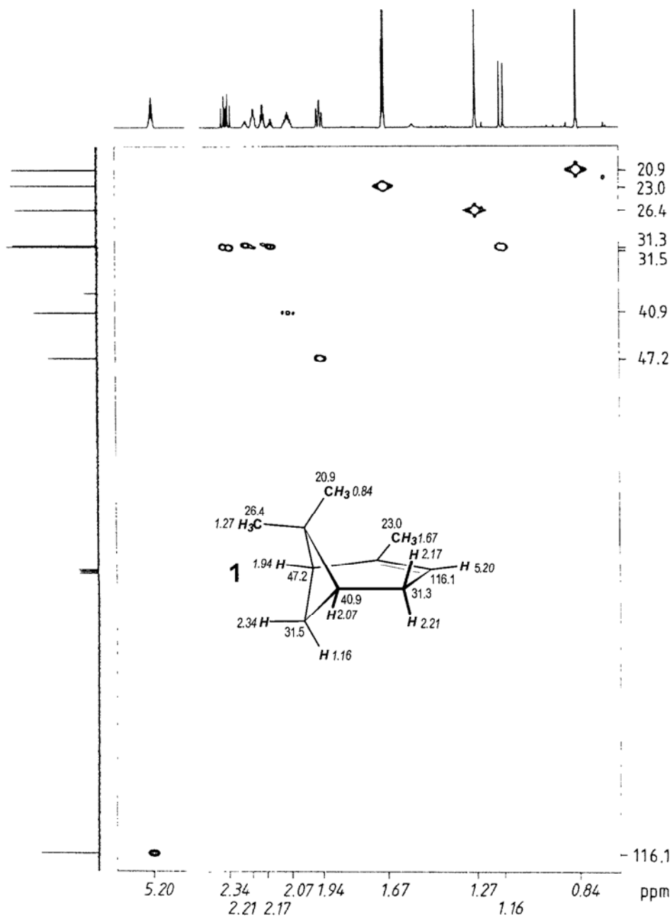
Figure 2.15. HC HSQC experiment (contour plot) of \alpha -pinene [(CDCl 3 , 5 % v/v, 25 °C, 125 MHz for ^{13}\text{C} , 500 MHz for ^1\text{H} , 4 scans, 256 experiments]. This experiment gives the same information as Fig. 2.14 within 8 minutes instead of two hours required for the CH-COSY in Fig. 2.14 due to higher sensitivity because of proton detection and stronger magnetic field. Deviations of proton shifts from those in Fig. 2.14 arise from the change of the solvent. The methylene protons collapsing in Fig. 2.14 at \delta_{\text{H}} = 2.19 (200 MHz) display in this experiment an AB system with \delta_{\text{A}} = 2.17 and \delta_{\text{B}} = 2.21 (500 MHz)
