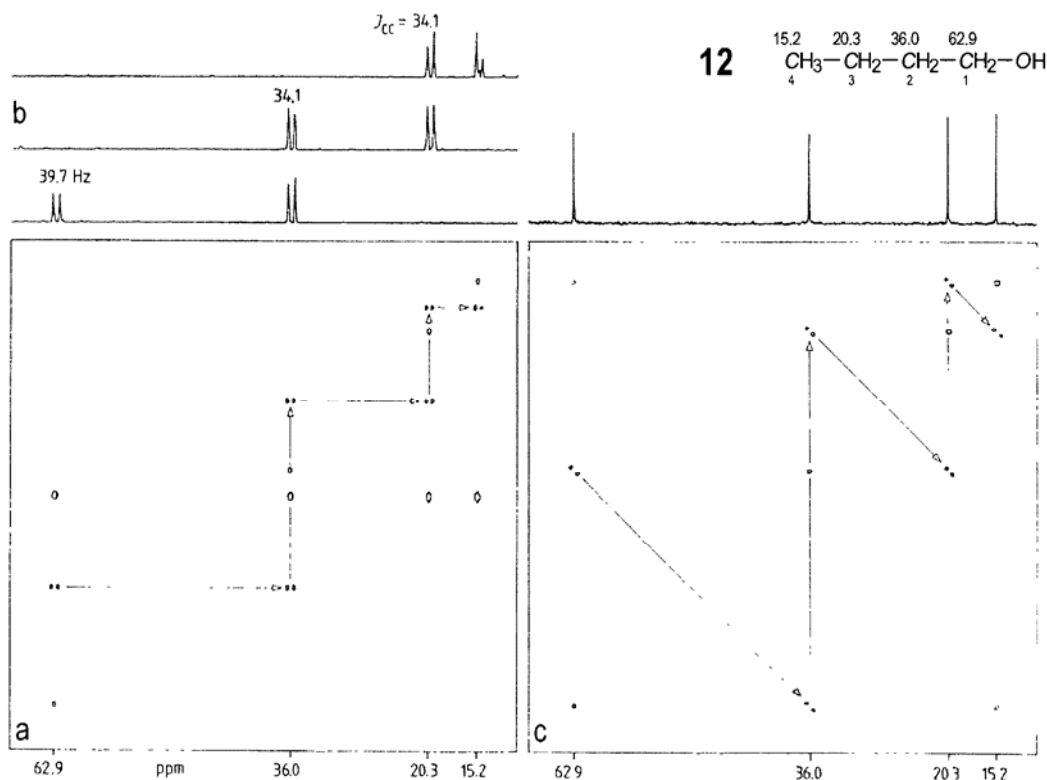
Figure 2.12. Two-dimensional (2D-)INADEQUATE diagram of 1-butanol ( 12 ) [(CD 3 ) 2 CO, 95% v/v, 25°C, 50 MHz, 128 scans, 128 experiments]. (a) Contour plot with the AB systems of bonded C atoms on the horizontal axis; (b) plots of the three AB systems of the molecule obtained from (a); (c) contour plot of the symmetrised INADEQUATE experiment showing the AB or AX systems of bonded C atoms in the HH COSY format (cross signals on the axes perpendicular to the diagonal)
