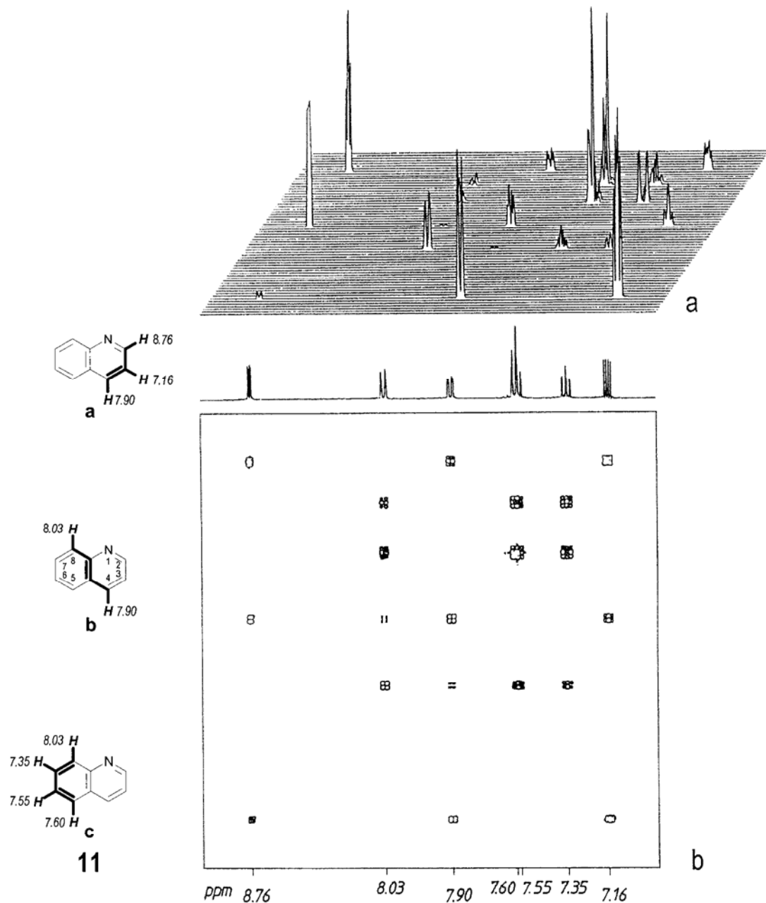
Figure 2.10. HH COSY diagram of quinoline (11) [( \text{CD}_3 ) _2\text{CO} , 95% v/v, 25°C, 400 MHz, 8 scans, 256 experiments]. (a) Stacked plot; (b) contour plot
