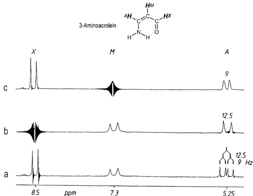
Figure 1.8. Homonuclear decoupling of the CH protons of 3-aminoacrolein ( \text{CD}_3\text{OD} , 25 °C, 90 MHz). (a) ^1\text{H} NMR spectrum; (b) decoupling at \delta_{\text{H}} = 8.5 ; (c) decoupling at \delta_{\text{H}} = 7.3 . At the position of the decoupled signal in (b) and (c) interference beats are observed because of the superposition of the two very similar frequencies
