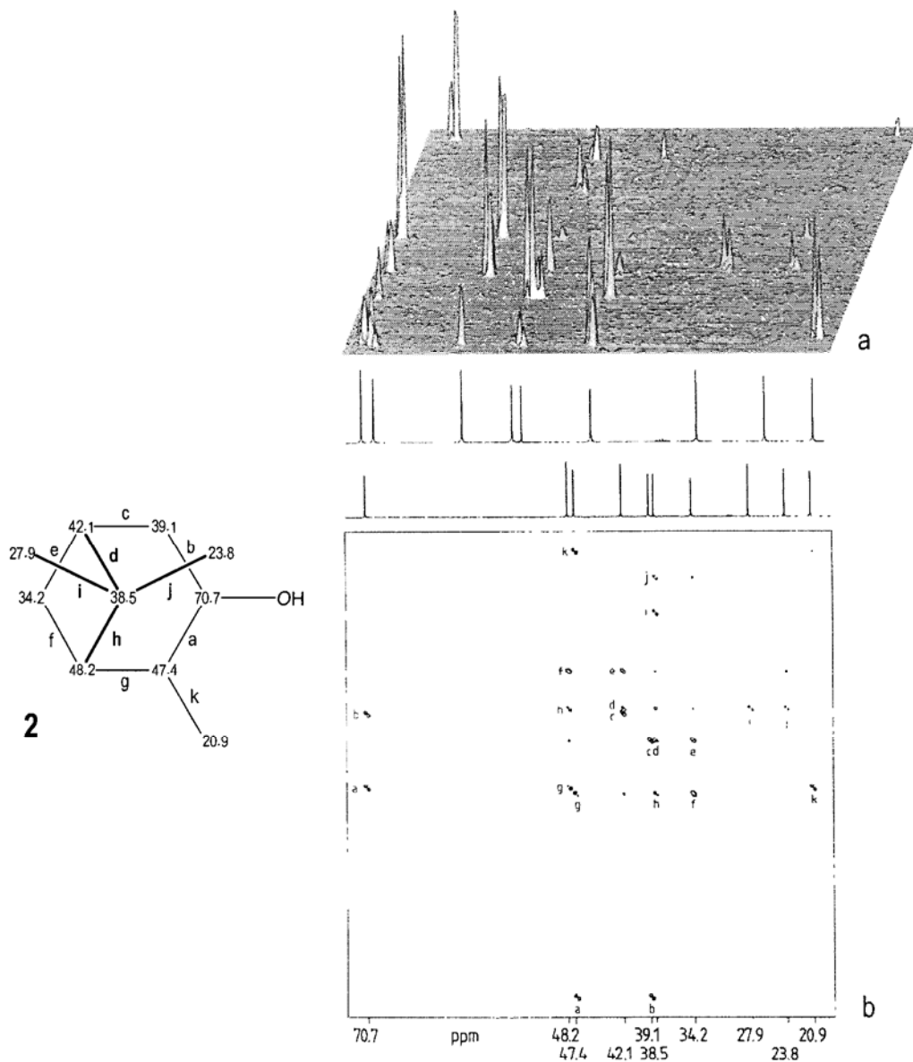
Figure 2.13. Symmetrised two-dimensional INADEQUATE experiment with isopinocampheol ( 2 ) [(CD 3 ) 2 CO, 250 mg in 0.3 ml, 25 °C, 50 MHz, 256 scans and exp.]. (a) Stacked plot of the section between δ c = 20.9 and 48.2; (b) complete contour plot with cross signal pairs labelled a-k for the 11 CC bonds of the molecule to facilitate the assignments sketched in formula 2
