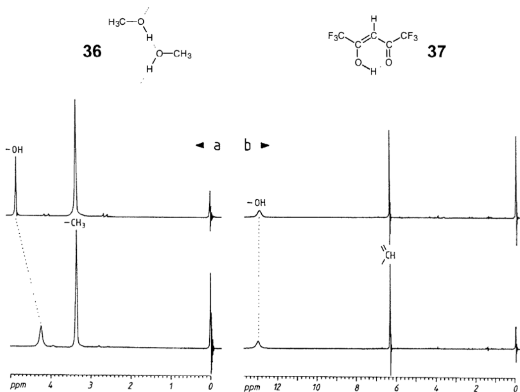
Figure 2.25. {}^1H NMR spectra of methanol ( 36 , a) and hexafluoroacetylacetone ( 37 , b), both in the pure state (above) and diluted in tetrachloromethane solution (5%, below) [25 °C, 90 MHz, CW recording]
