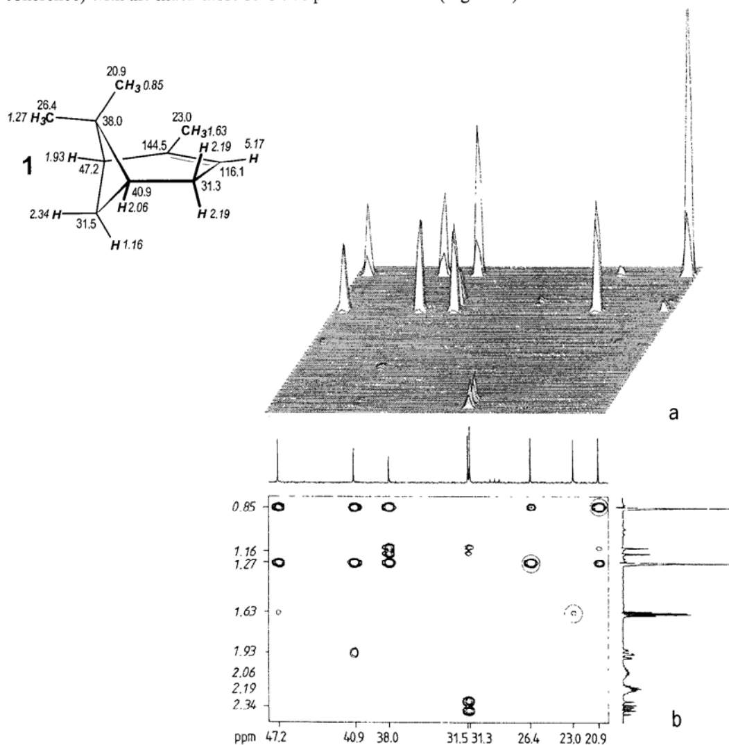
Figure 2.16. CH COLOC experiment of \alpha -pinene [( \text{CD}_3 ) _2\text{CO} , 10% v/v, 25 ^\circ\text{C} , 50 MHz for ^{13}\text{C} , 200 MHz for ^1\text{H} , 256 scans and experiments]. (a) stacked plot of the section between \delta_{\text{C}} = 20.9 and 47.2 ( ^{13}\text{C} ) and \delta_{\text{H}} = 0.85 and 2.34 ( ^1\text{H} ); (b) contour plot of (a). One-dimensional ^{13}\text{C} and ^1\text{H} NMR spectra for this section are shown aligned with the abscissa and ordinate of the contour plot. ^1J_{\text{CH}} correlation signals which are already known from the CH COSY study (Fig. 2.14) and have not been suppressed, are indicated by circles
