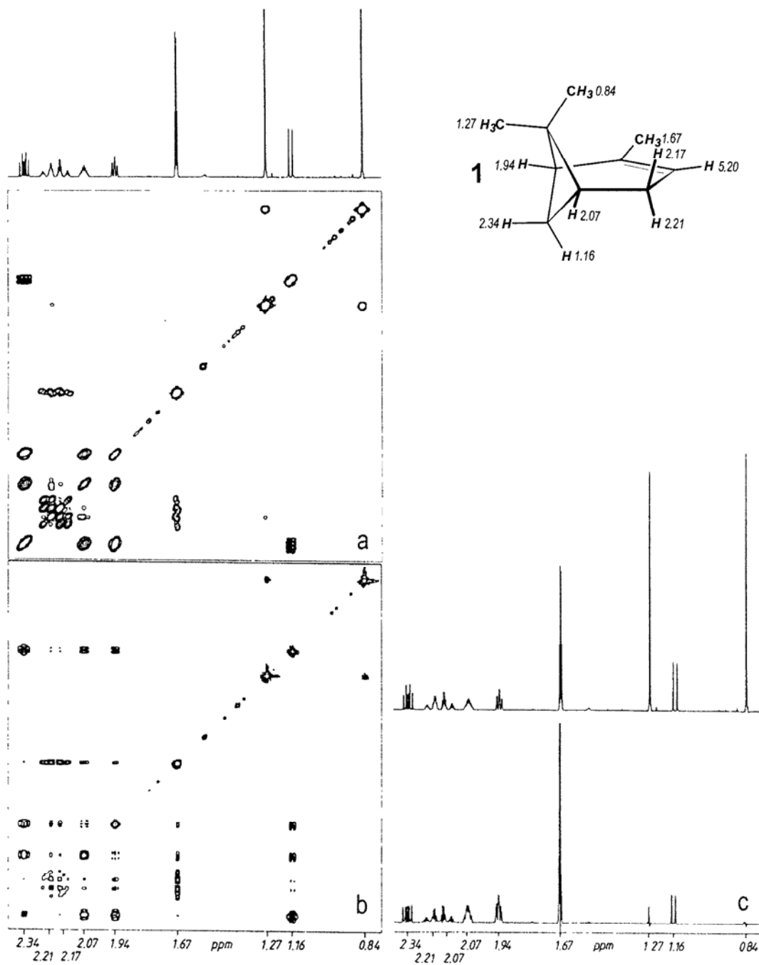
Figure 2.11. Proton-Proton shift correlations of \alpha -pinene (1) [purity 99 %, CDCl_3 , 5 % v/v, 25 °C, 500 MHz, 8 scans, 256 experiments]. (a) HH COSY; (b) HH TOCSY; (c) selective one-dimensional HH TOCSY, soft pulse irradiation at \delta_H = 5.20 (signal not shown), compared with the ^1H NMR spectrum on top; deviations of chemical shifts from those in other experiments (Fig. 2.14, 2.16) arise from solvent effects
